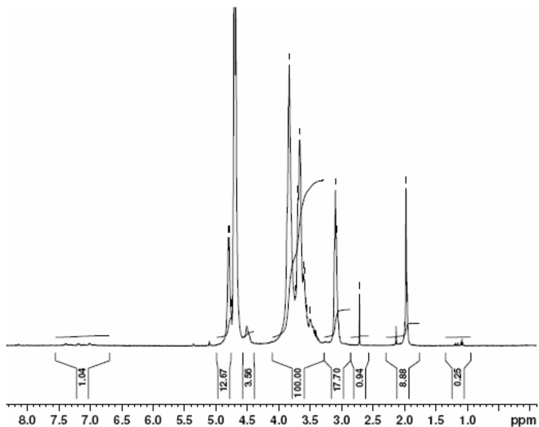
H-NMR Spectrum of Chitosan-FITC polymer in H 2 O (Varian Inova 500 MHz instrument)
